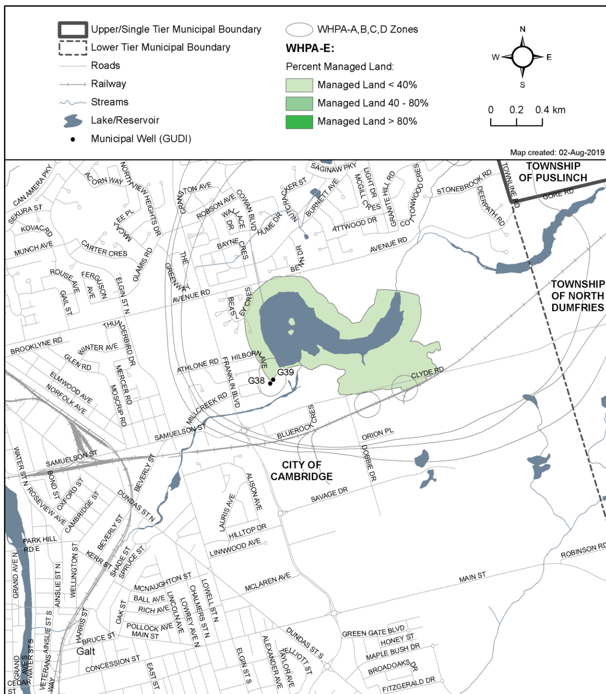
Map 8.5—25: Shades Mills Wellfield Percent Managed Lands- WHPA-E
