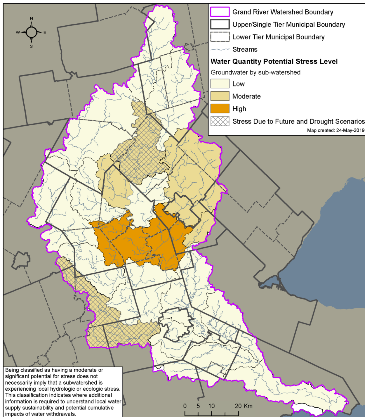
Map 18-4: Water Quantity Stress Levels by Groundwater Assessment Area within the Grand River Watershed
